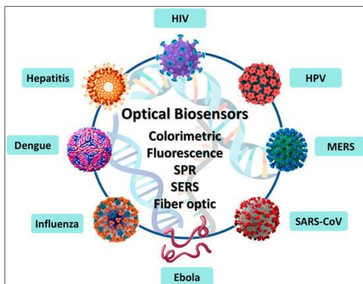
Figure 2 Optical/Visual Biosensors
