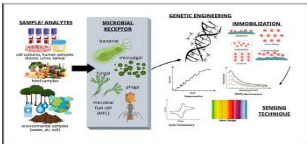
Figure 5 Microbial Biosensors
