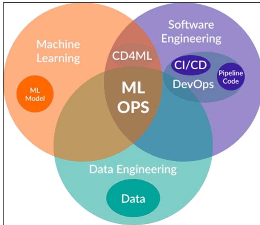
Figure 2 MLOps
