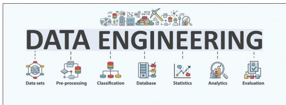
Figure 1 Data Engineering
